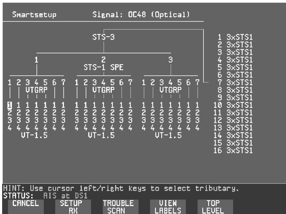
Figure 14.33 SDH/SONET testing using a portable SDH/SONET analysis system
