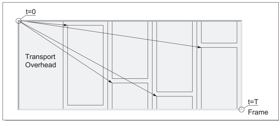
Figure 14.29 SDH/SONET pointers
