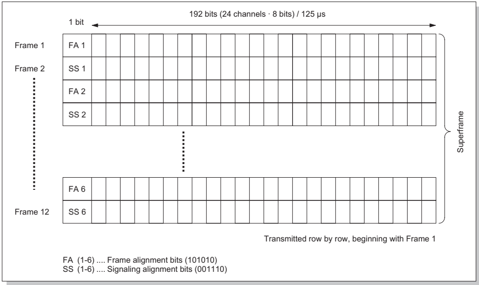
Figure 14.2 DS1 superframe
