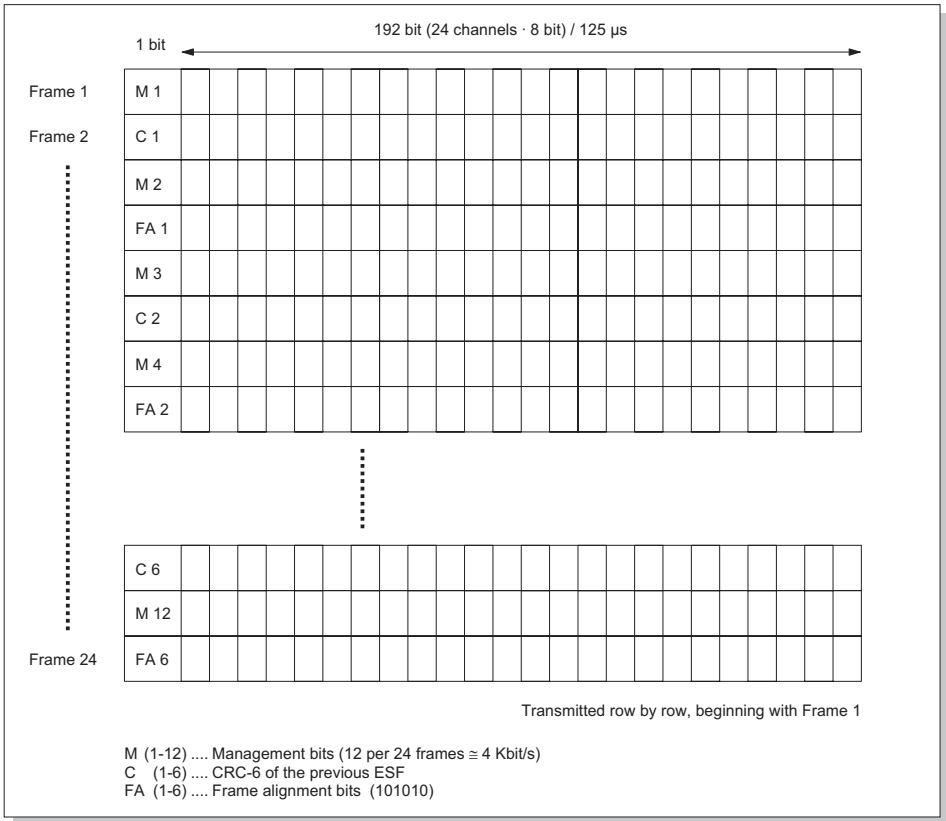
Figure 14.3 DS1 extended superframe (ESF)
