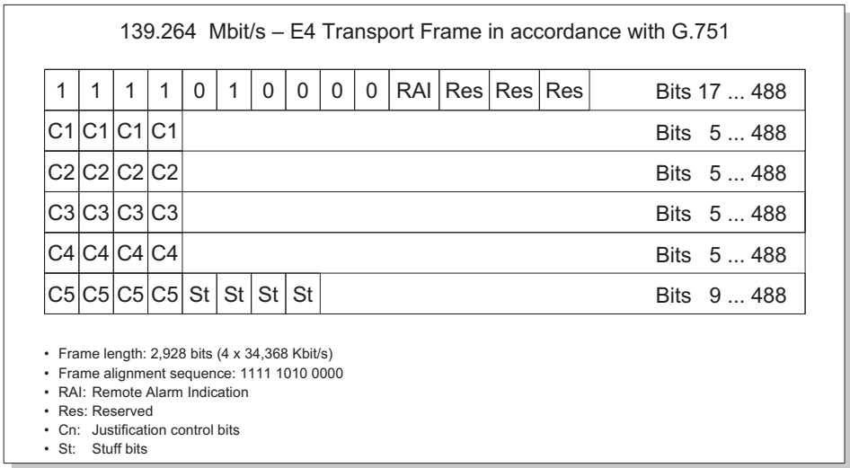
Figure 14.14 E4 frame
