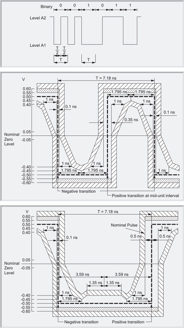
Figure 14.15 Pulse mask for the E4 interface
