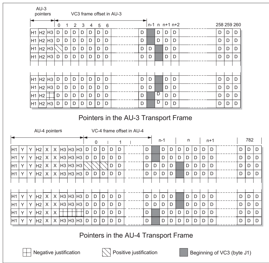
Figure 14.30 AU4 pointer adjustment (VC-4 in STM-1)
