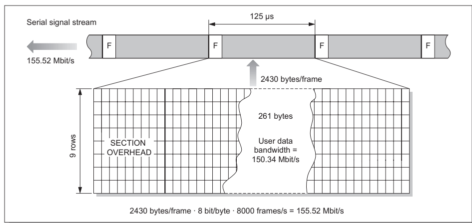
Figure 14.19 STS-3c/STM-1 frame
