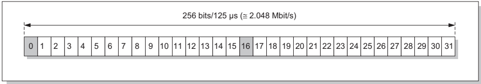
Figure 14.5 E1 frame
