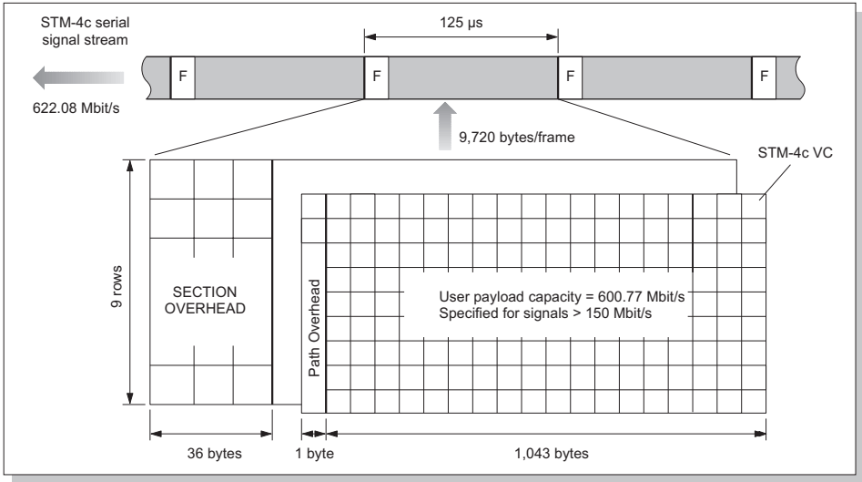
Figure 14.26 STM-4c transport module
