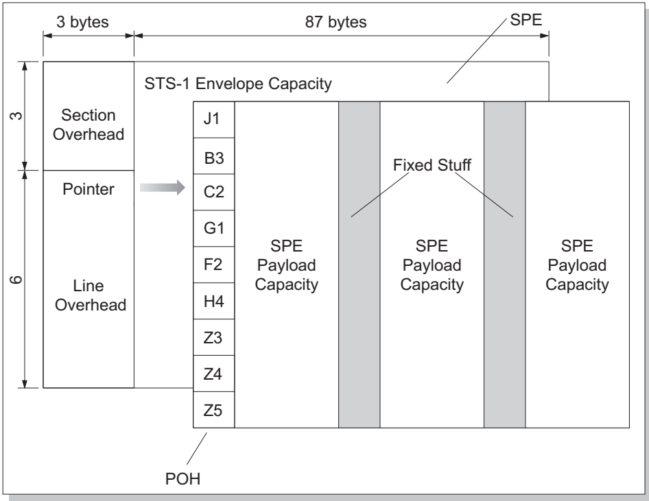
Figure 14.18 STS-1 frame
