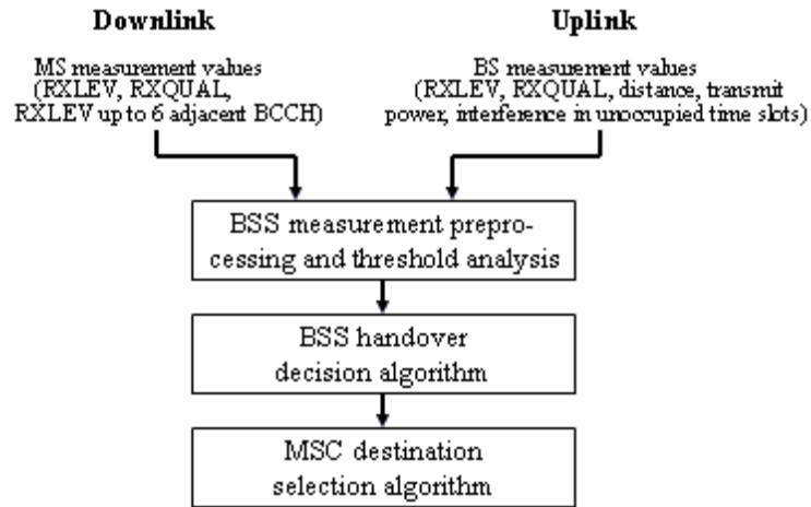
Figure 3: Decision steps in a GSM handover
